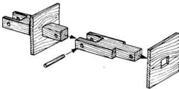
Typical wooden paddle and chain design
